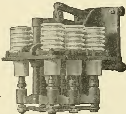
Fig. 156. Rear View Hand-Operated 300-Ampere, 3-Pole Circuit Breaker. Closed Position
